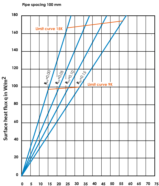
Nominal heating medium differential temperature \Delta t in K = Average heating water temperature minus room temperature
